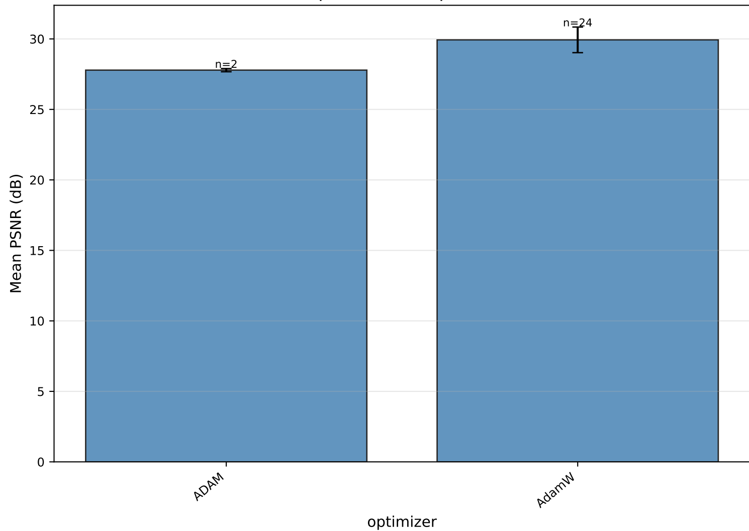
Mean PSNR per value of optimizer — SwinT
